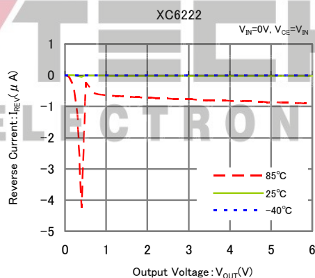
(7) Reverse Current vs. Output Voltage
