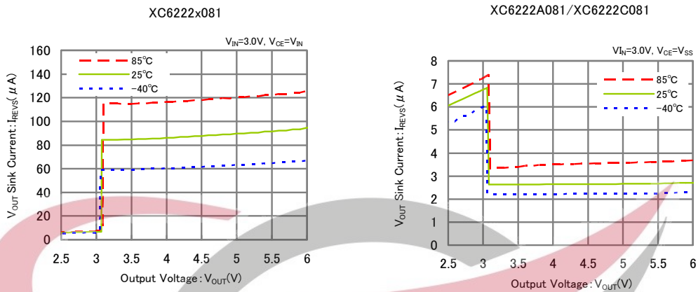
(8) V_{OUT} Sink Current vs. Output Voltage
